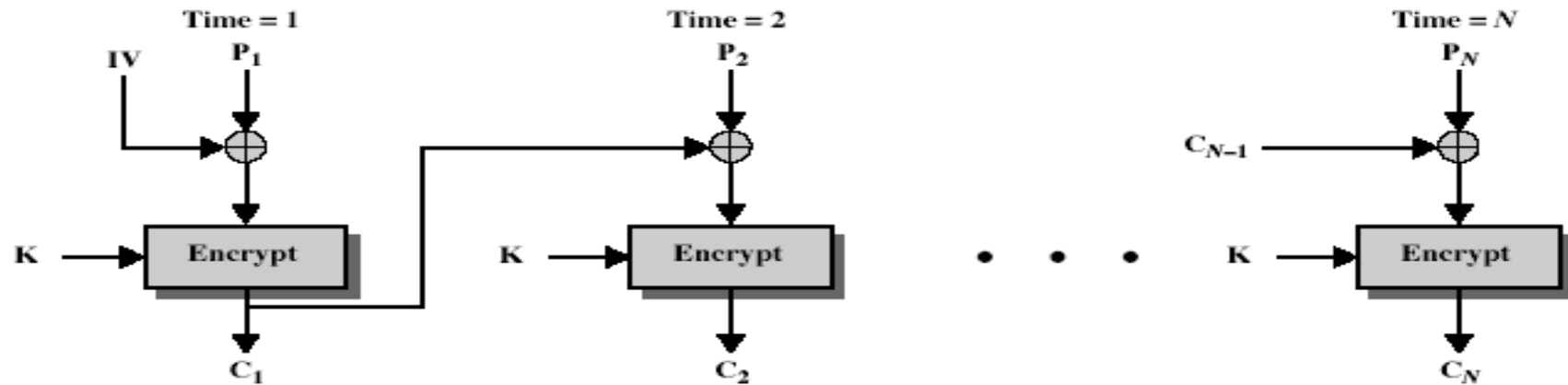
(a) Encryption
