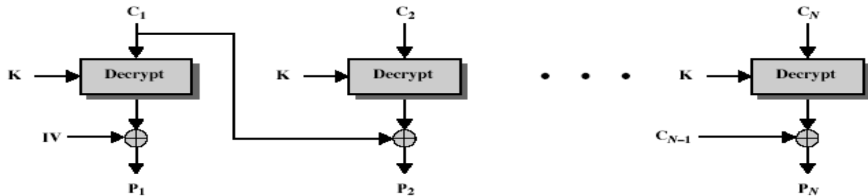
(b) Decryption
