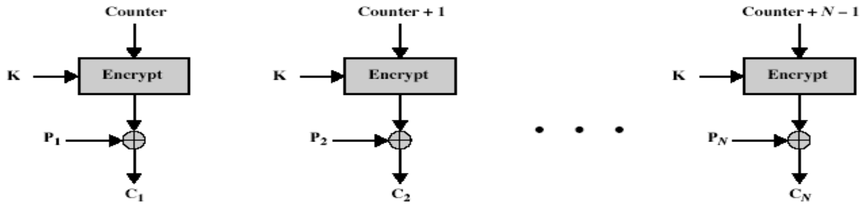
(a) Encryption
