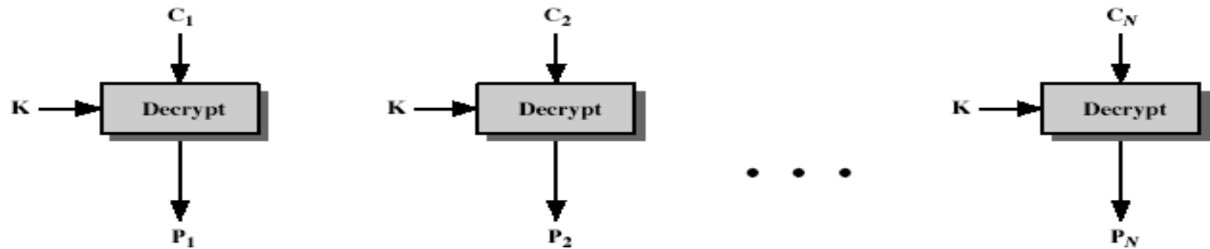
(b) Decryption
