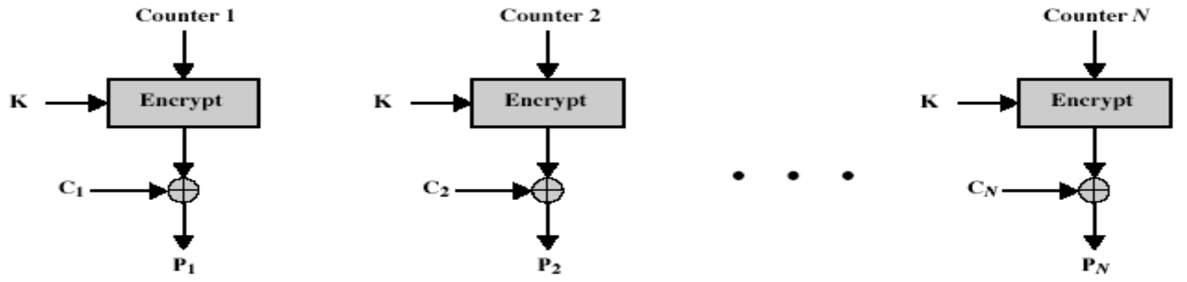
(b) Decryption
