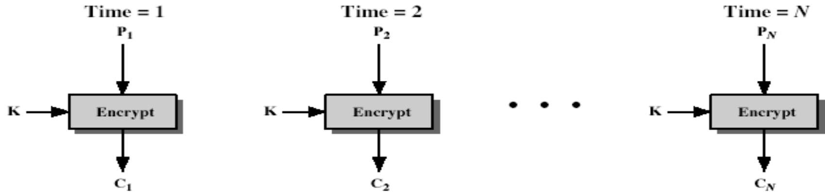
(a) Encryption
